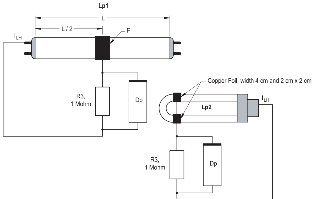
Figure 8.7 Detection of lamp current (See Clauses 8.17.4.4.1 and 8.17.4.4.2)
