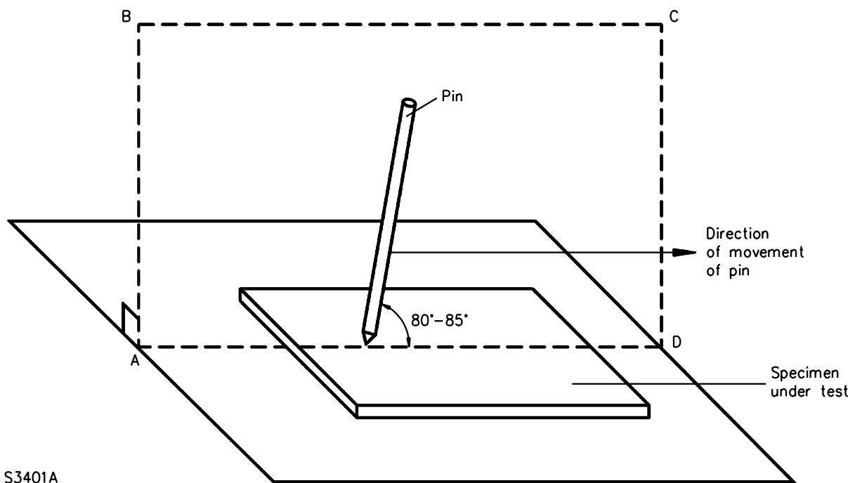
Figure E.1 Abrasion resistance test apparatus for PCB conformal coatings (See Clauses E.3.2.3 and E.3.3.1)
