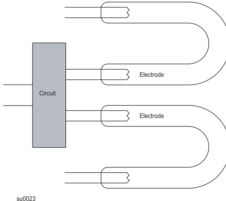
Figure 8.2 Fault conditions test diagram (See Clause 8.16.2)
