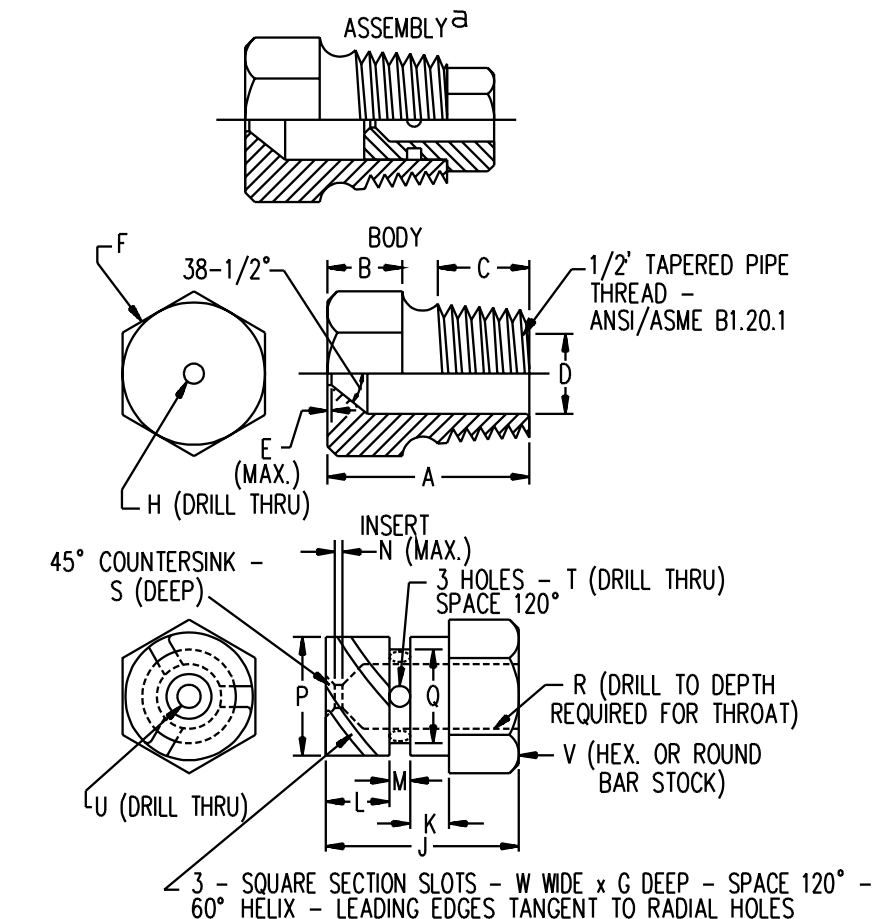
Figure 9.4 Spray head assembly (See Clause 9.7.1)
