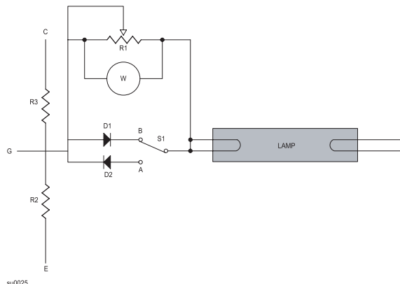
Figure 8.4 Asymmetric power test schematic (See Clause 8.17.3.1)
