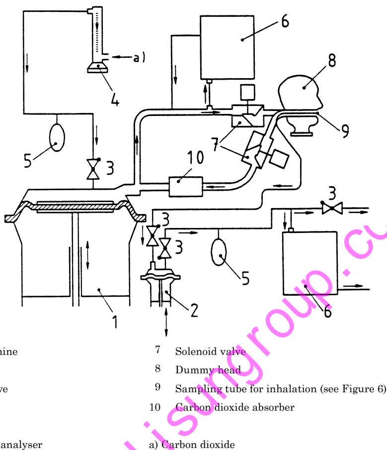
Figure 7 — Arrangement for testing carbon dioxide content of the inhalation air
